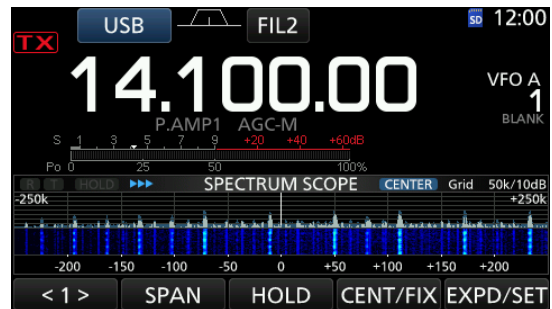
SPECTRUM SCOPE-Fenster
