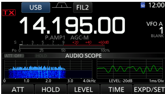
AUDIO SCOPE-Fenster
