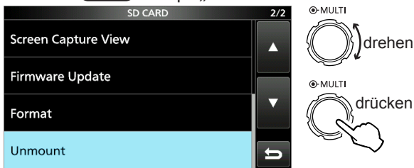
SD CARD-Fenster
