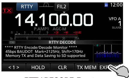
RTTY DECODE-Fenster
